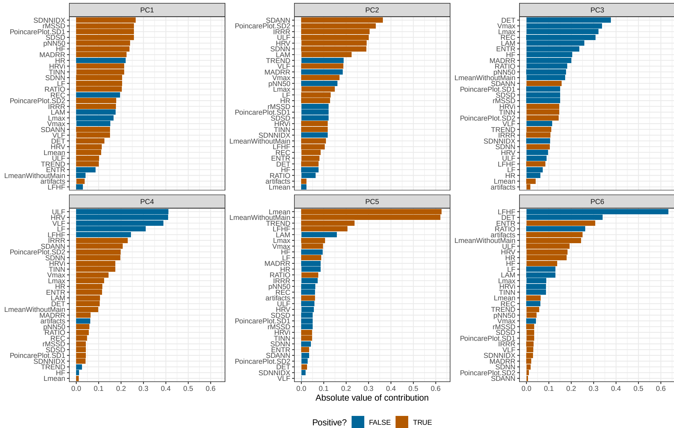
Loadings plot of the first 6 principal components of PCA for FLARE008
